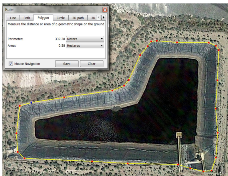
Figure 30. Estimating the area of a dam
