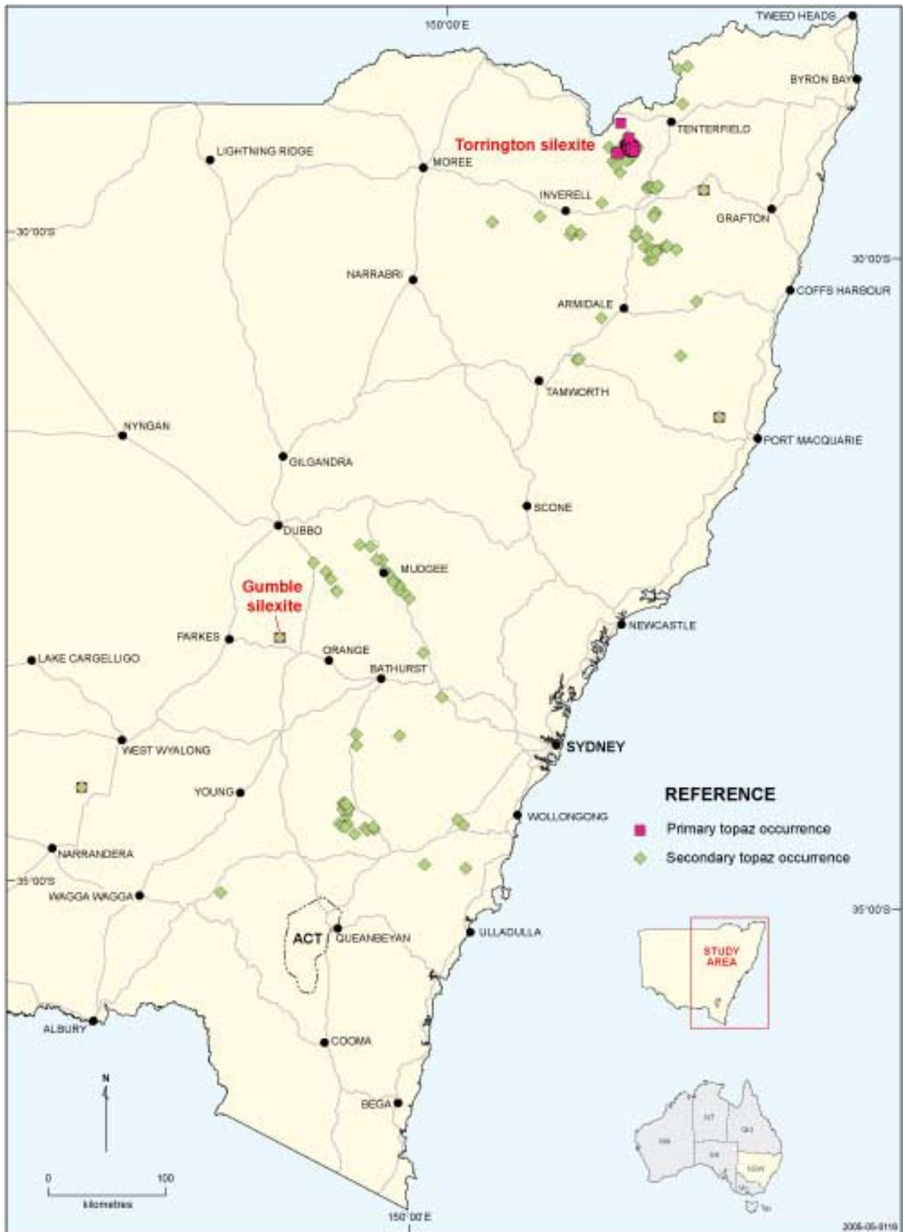
Figure 29. Topaz occurrences in eastern New South Wales
