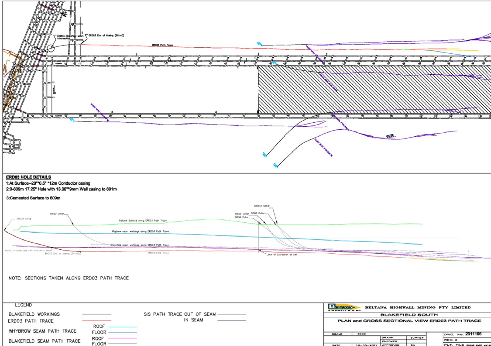
Figure 30: Cross-section View of ERD03
