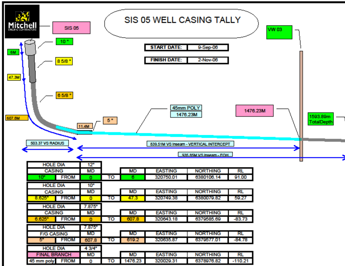
Figure 31: SIS05 Well Casing Tally
