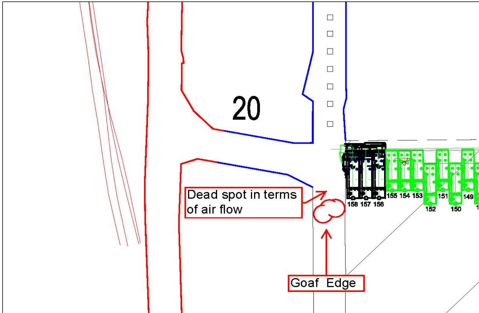
Figure 7: Enlargement of tailgate at 20 C/T highlighting goaf edge and dead spot in the ventilation
