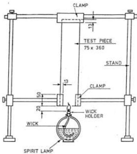
Figure 5 Experimental set up for the spirit lamp and follow up flame tests
