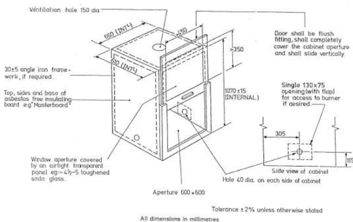
Figure 3 Schematic diagram of cabinet
